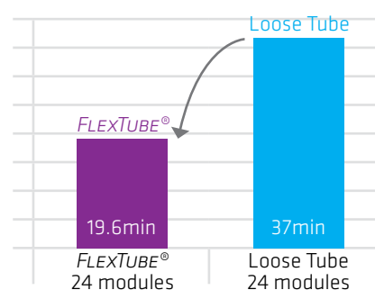
Mid Span Access: 6 modules out of 24 prepared, the 18 left coiled
