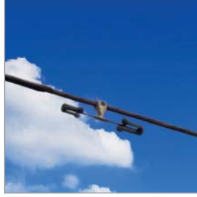
2 Stockbridge damper
