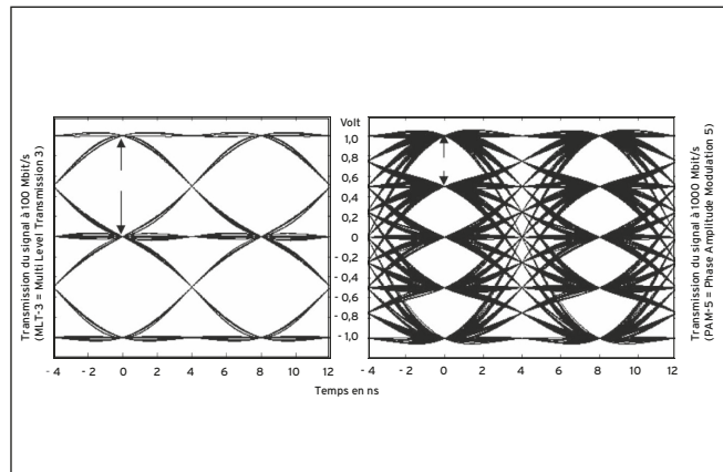
Signaltransmission at 100 Mbit/s and 1000 Mbit/s
